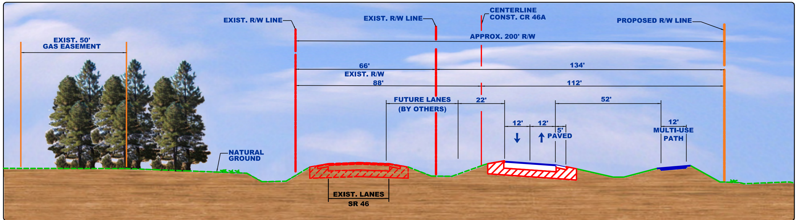
TYPICAL SECTION From Sorrento Avenue To Wekiva Trail Trailhead
