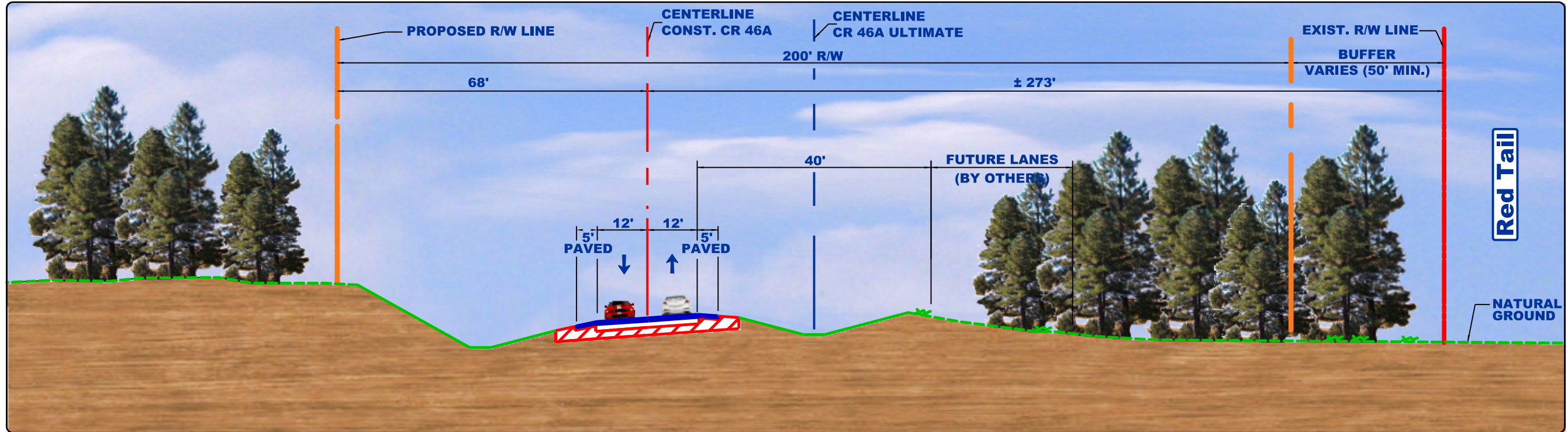
TYPICAL SECTION From Arundel Way to Sorrento Avenue
