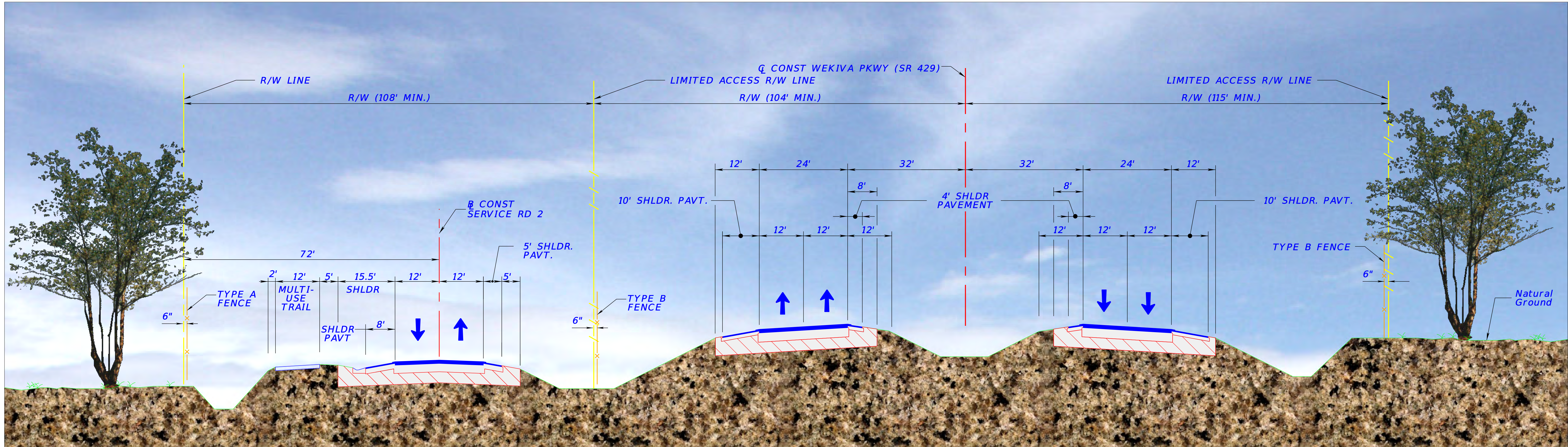
TYPICAL SECTION
